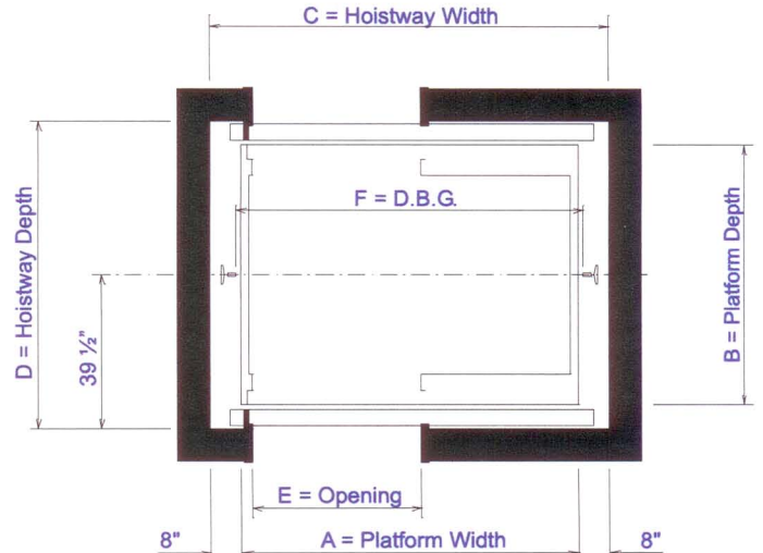
Hoistway Figure 2: "Front & Rear Openings"
