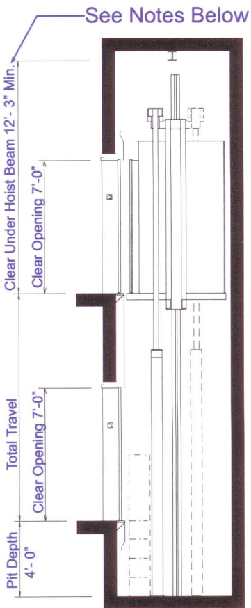
Hoistway Figure 1: "Front Opening Only"
