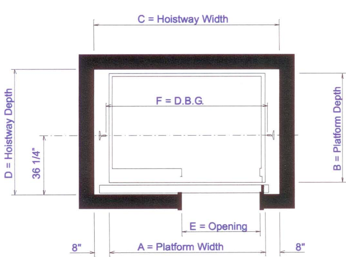
Hoistway Figure 1: "Front Opening Only"
