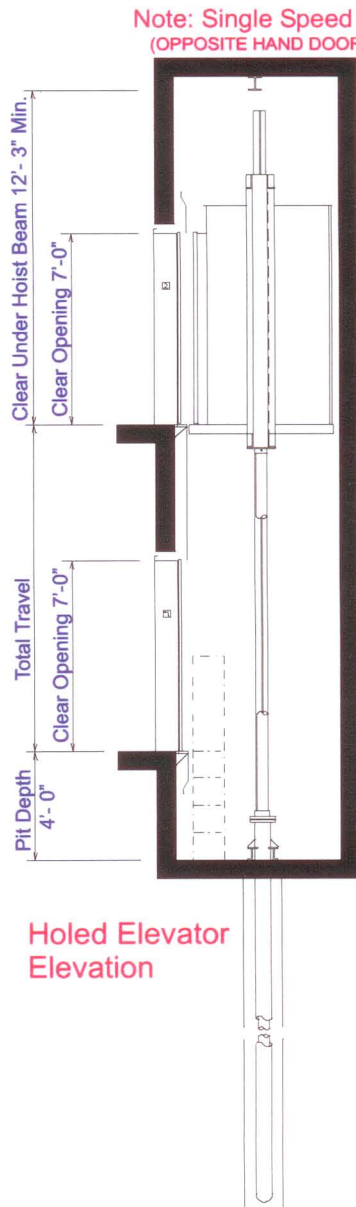
Hoistway Figure 1: "Front Opening Only"
